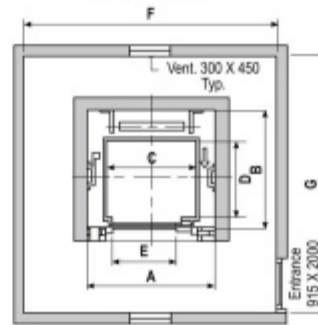
Hoistway Machine Room Plan For Manual Door
