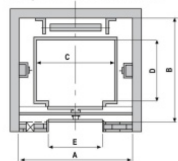
Hoistway Machine Room Plan For Auto Door
